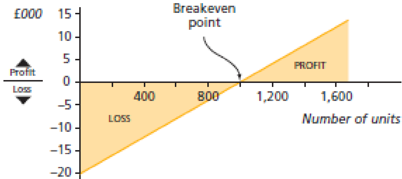
Figure 4.3 Profit-volume chart
